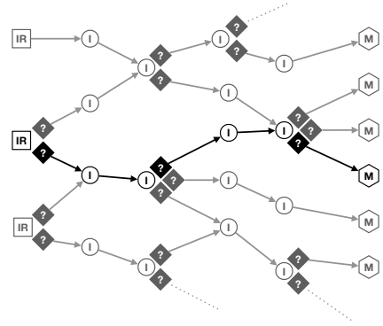
Fig. 1. Conceptual graph visualization of ISLE programs mapping IR terms \boxed{\text{IR}} via intermediate terms \textcircled{I} to machine code (ISA) terms \boxed{\text{M}} . Rule match conditions use \blacklozenge predicates, often via a bridge to external Rust.
