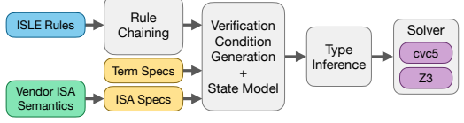
Fig. 3. ARRIVAL's verification pipeline.
