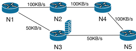
Figure 2: Composition scenario: two applications to be deployed and their optimizations to be applied to Web and SSH traffic (respectively).
