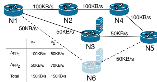
Figure 5: Traffic shift from time epoch e_1 to e_2 causes a policy violation if path N_1 - N_6 - N_5 is not chosen, despite the total volume of traffic remaining the same.
