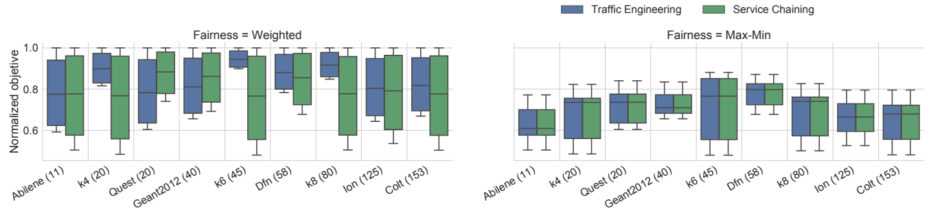
Figure 13: Impact of chosen fairness metric on the objective function of each application
