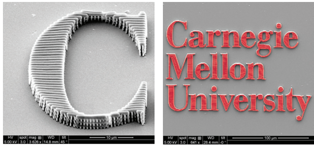
Log-pile nanostructure using a Nanoscribe 3-D printer Conceptualized at 1:00 am and printed at 2:15 am – Metin Gökhan Güney, Ph.D. candidate
