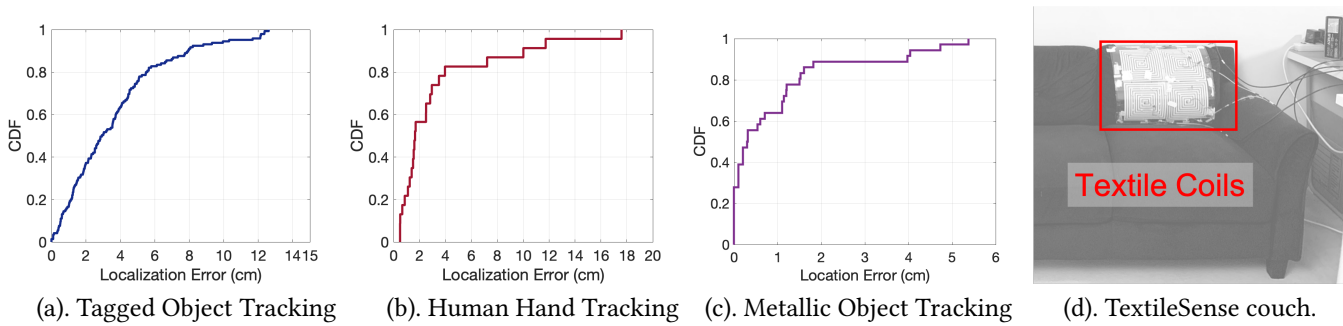
Figure 8: CDF of localization accuracy for (a) NFC-tagged object, (b) human hand, (c) untagged metallic object. (d) Example Application Setup.
