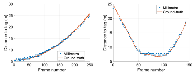
Figure 16: Millimetro's ranging under mobility
