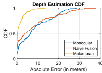
Fig. 7. CDF of depth errors shows our depth estimation at long ranges in clutter.
