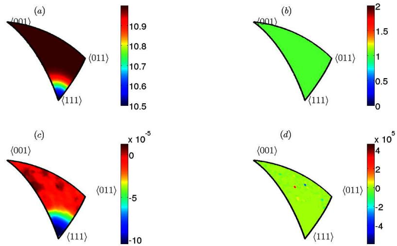
Figure 6.33: (a) Theoretical energy density \gamma in the repeating triangular subregion delineated by the \langle 001 \rangle , \langle 011 \rangle and \langle 111 \rangle axes; (b) Theoretical mobility \mu (constant) in the same region; (c) computed energy density, (d) computed mobility.
