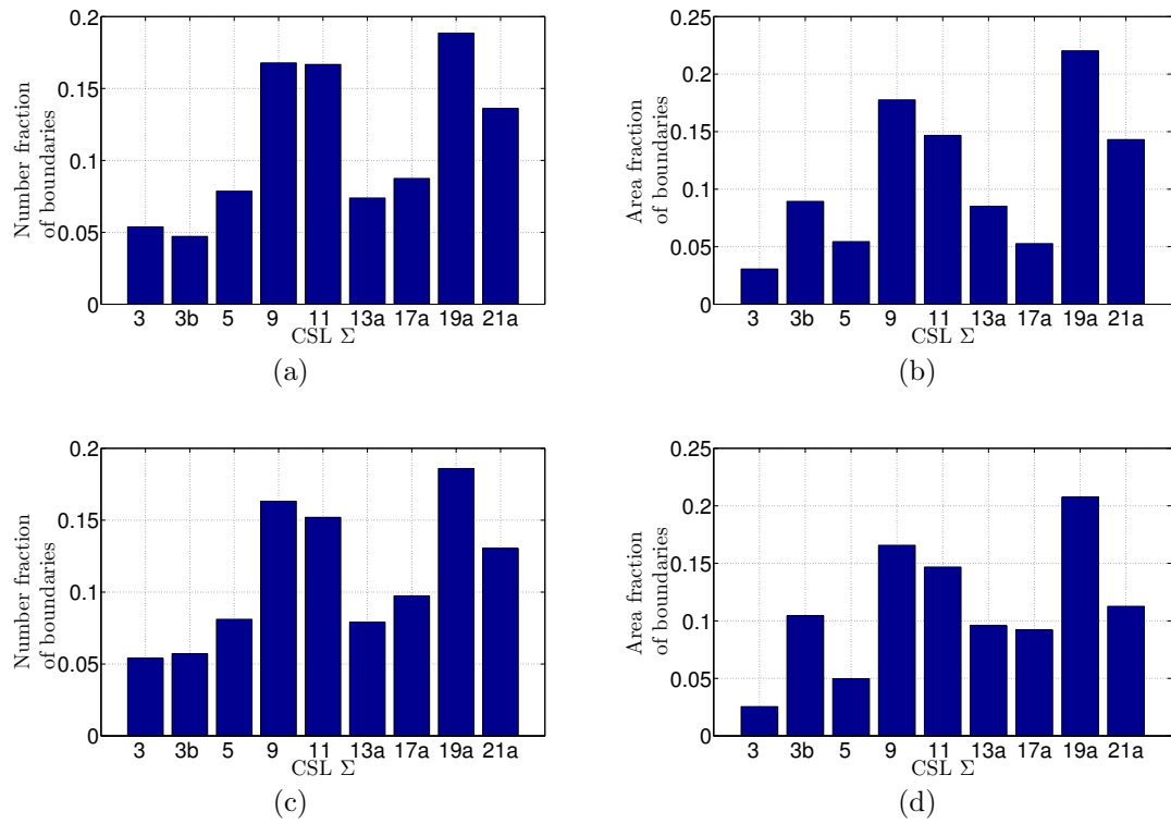
Figure 6.19: Number fractions of grain boundaries for select CSL disorientations: Left: Number fraction of boundaries, Right: Area fraction of boundaries, Top: pre-anneal volume, Bottom: post-anneal volume.
