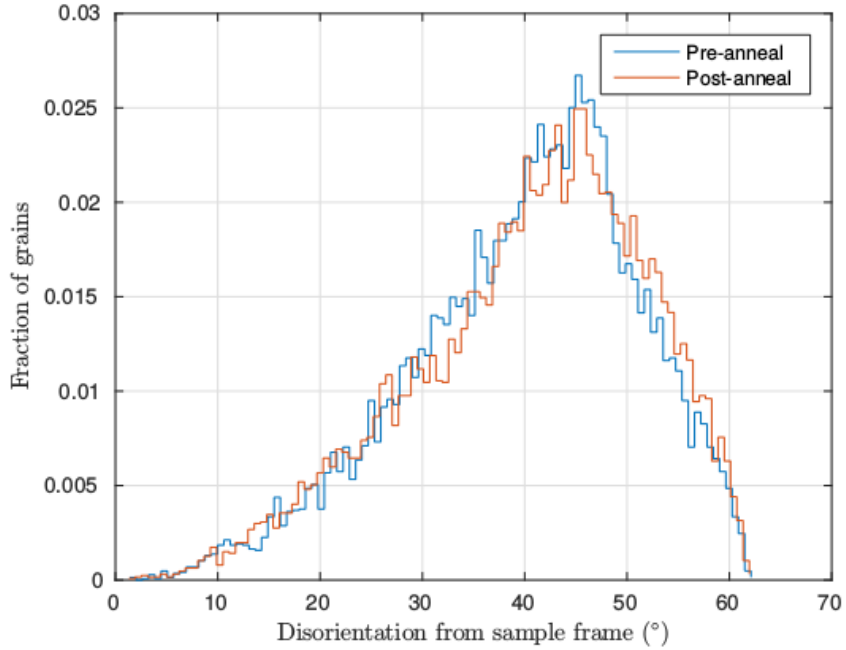
Figure 6.5: Distributions of the angle of disorientation of the grain lattices form the sample frame, before and after anneal. In both cases the distribution is shown to follow the Mackenzie distribution.
