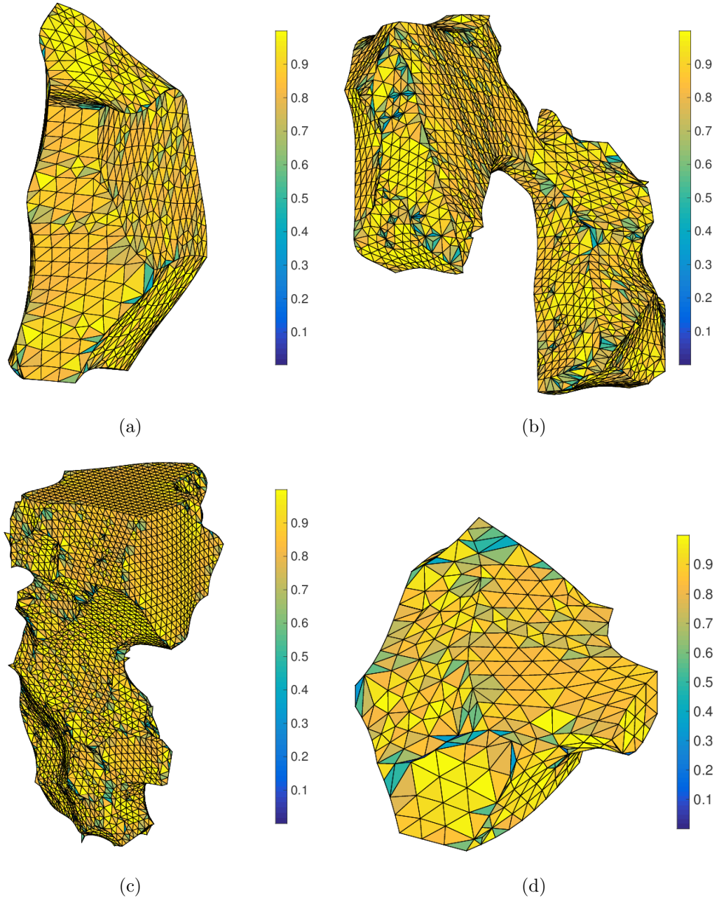
Figure 4.10: Mesh quality of select grains in the microstructure volume. The grain in (d) is the same as the one in Figure 4.7.
