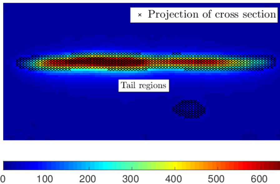
Figure 3.5: Estimating the projection of the cross section of grains by eliminating the surrounding tail regions from the intensity profile. The color scale denotes the pixel-wise intensity count returned by the CCD camera while the 'x' markers are those pixels estimated by the edge detection algorithm to be inside the geometric projection of the grain.
