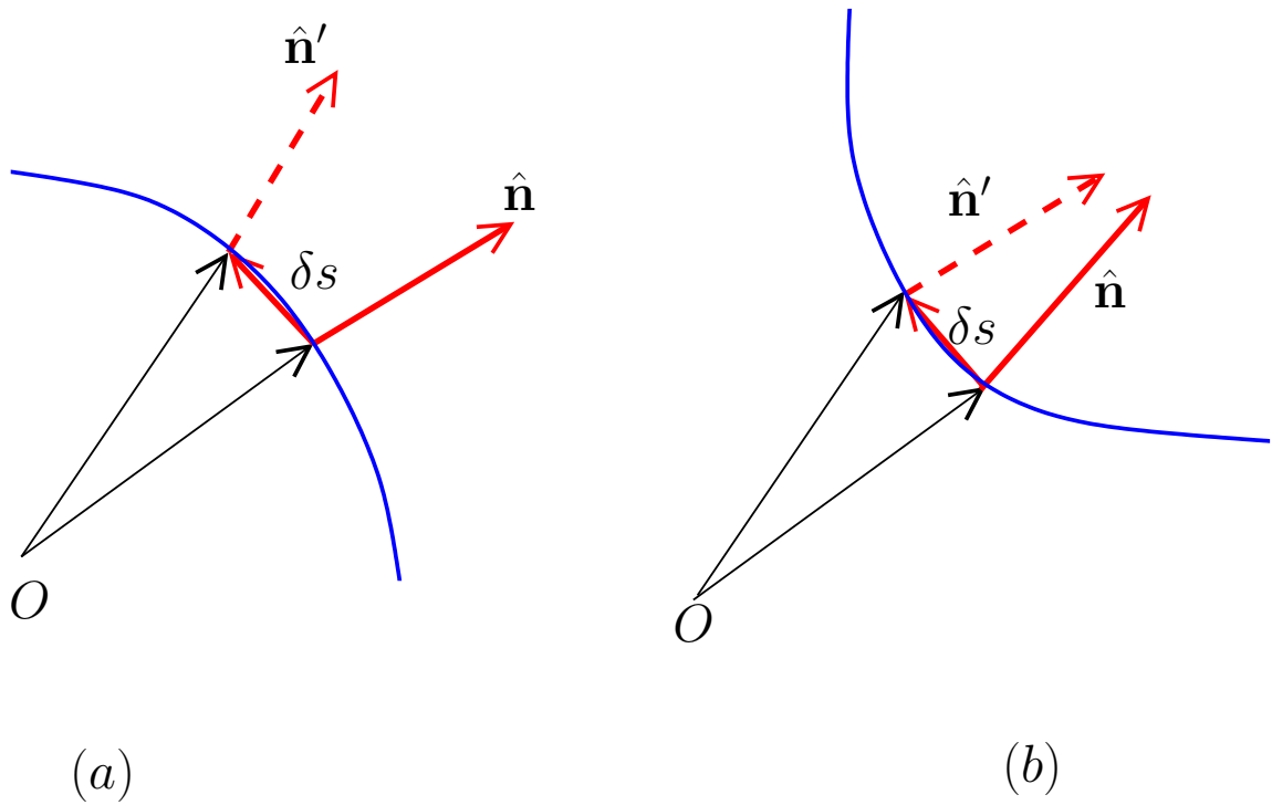
Figure 6.24: (a) positive curvature, (b) negative curvature.
