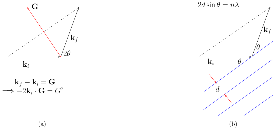
Figure 2.4: (a) Illustration of the von Laue condition for non-zero scattering in reciprocal space, (b) the equivalent Bragg condition in real space, with the reflecting atomic planes shown in blue.
