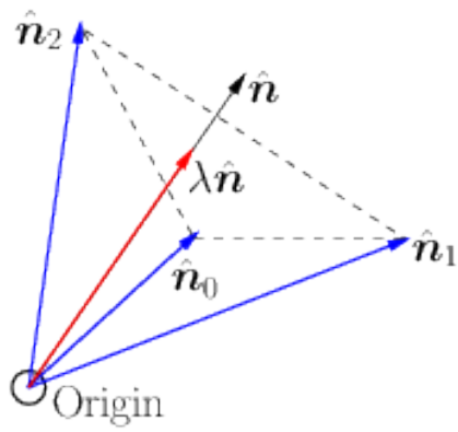
Figure 5.5: The condition for \hat{n} to lie inside the solid angle subtended by \{\hat{n}_0, \hat{n}_1, \hat{n}_2\} : The vector \lambda \hat{n} lies inside the triangle bound by \{\hat{n}_0, \hat{n}_1, \hat{n}_2\} for some \lambda > 0 .
