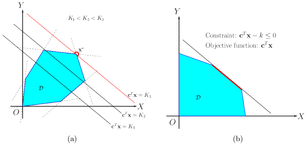
Figure 3.9: (a) A two-dimensional case of linear optimization with the feasible region \mathcal{D} shown in shaded color. c^T \mathbf{x} = K denotes the family of straight lines represented by the objective function, whose value K is to be maximized. The maximum value of K that falls in the feasible region is precisely at the maximizer \mathbf{x}^* , which is a vertex of the simplex. (b) A case of an ill-posed problem in which the expression for one of the linear constraints is the same as the linear objective function. In this case the maximizer is not unique, in fact every point on the red line is a solution to the problem.
