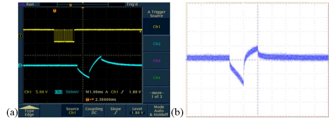
Fig. 9. Typical electrode voltage waveforms (a) when the stimulator drove a dummy load consisting of a series resistor of 4 k \Omega (representing the access resistance and the series resistance of the lead), and a parallel combination of a 20 k \Omega resistor and a 0.047 \mu\text{F} capacitor representing the electrode–tissue interface (the top trace shows the binary bitstream used to command the device and the bottom trace shows the voltage output.) (b) Representative electrode voltage waveform when the stimulator was wirelessly powered in saline solution, measured using a “test tail” extension of the IrO x electrode array that reached back out of the bath. The noise is due to RF interference from the transmitter.
