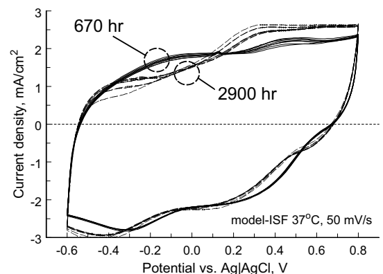
Fig. 6. Cyclic voltammograms of eight SIROF electrodes after 670 hr (solid) and 2900 hr (dashed) of pulsing at 200 \mu\text{C}/\text{cm}^2 .
