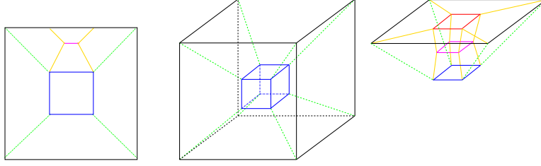
Fig. 9. Adaptive hexahedral mesh decomposition (Method 1). Left - a 2D example; Middle - a small hexahedron is inserted; Right - the top face of the original hexahedron needs to be refined, 6 hex and 8 extra vertices are generated.
