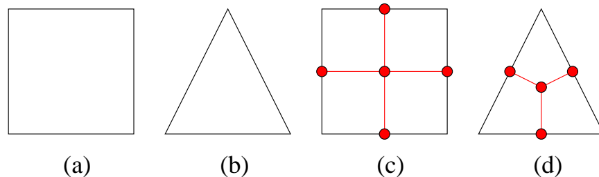
Fig. 3. The templates to decompose a quad or a triangle into quads. Red points are newly inserted at the middle of edges or the element center. (a) - a quad before splitting; (b) - a triangle before splitting; (c) - a quad is split into four quads; (d) - a triangle is split into three quads.
