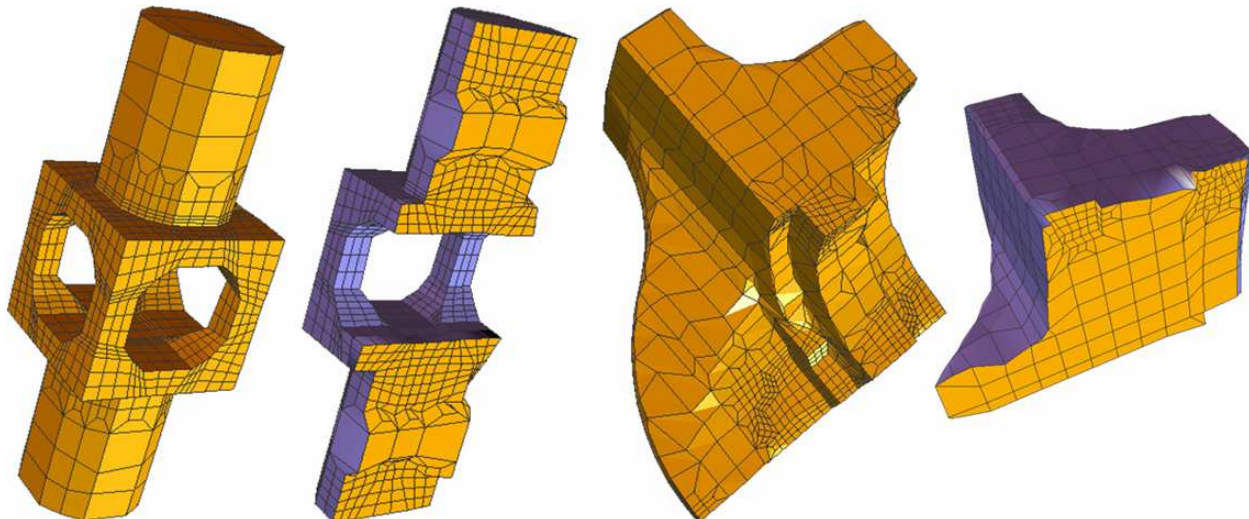
Fig. 14. Sharp features are preserved. From left to right: an adaptive quad mesh of a mechanical part, an adaptive hex mesh of a mechanical part, an adaptive quad mesh of a fan disk, and an adaptive hex mesh of a fan disk.
