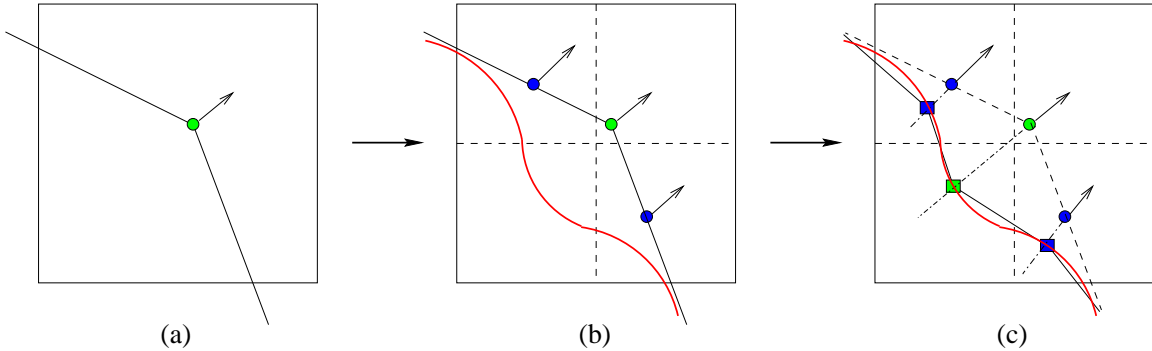
Fig. 6. The calculation of vertex positions. (a) - one leaf cell; (b) - the leaf cell is subdivided into four subcells, and three minimizer points are obtained; (c) - the three minimizer points are moved to the isocontour along their normal directions. The red curve is the real isocontour. The green circle point represents an existing minimizer point of this leaf cell, and blue circle points are two newly inserted vertices. The arrows are their normal vectors, the green and blue box points are the resulting vertices.
