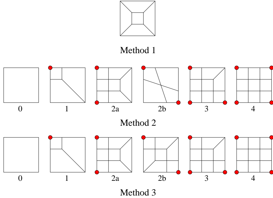
Fig. 4. Three different methods to define templates for adaptive quadrilateral isosurface extraction. In Method 1, the quad needs to be refined; In Method 2 and 3, octree leaf cells generating red minimizer points need to be refined.
