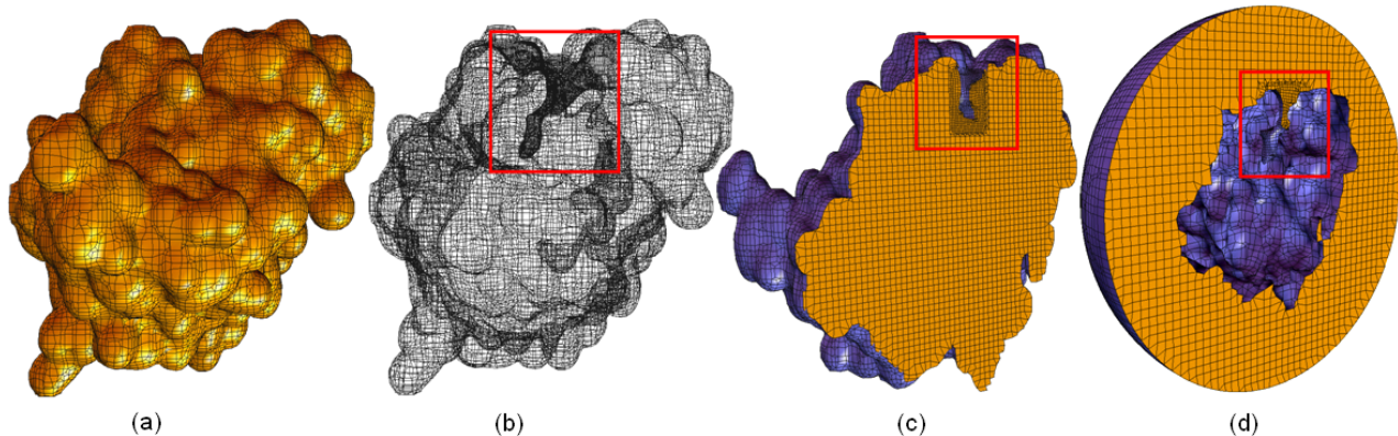
Fig. 1. Adaptive quadrilateral and hexahedral meshes of a biomolecule mAChE. (a) - the quadrilateral mesh of the molecular surface; (b) - the wireframe of the adaptive quadrilateral mesh of the molecular surface; (c) - the adaptive hexahedral mesh of the interior volume; (d) - the adaptive hexahedral mesh of the exterior volume between the molecular surface and an outer sphere. Finer meshes are generated in the region of the cavity, while coarser meshes are kept in other areas. The cavity is shown in the red boxes.
