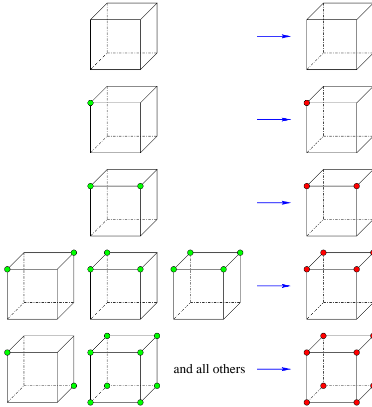
Fig. 12. The Look-Up table for converting an arbitrary configuration to one of the five templates in Figure 10. Each green node represents the cell from which the minimizer point is generated needs to be refined. The sign of the cell generating a red node is 1, otherwise the sign is 0.
