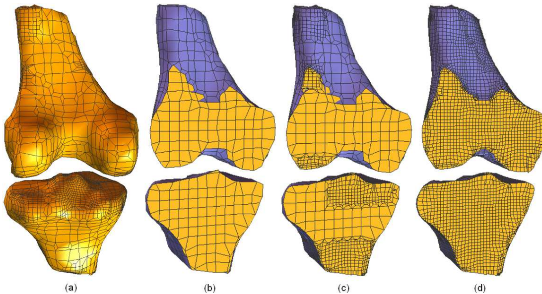
Fig. 19. Quadrilateral and hexahedral meshes of the knee. (a) - an adaptive quadrilateral mesh; (b) - the uniform hexahedral mesh at a chosen starting level; (c) - an adaptive hex mesh controlled by the feature sensitive error function; (d) - all the hexahedral elements in (b) are refined.
