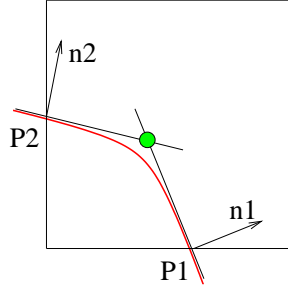
Fig. 2. The quadratic error function (QEF) and the minimizer point in 2D. The red curve is an isocontour, and the green point is the minimizer point calculated in Equation 1. (p_1, n_1) and (p_2, n_2) represent the position and unit normal vectors of the two intersection points.
