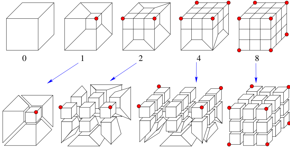
Fig. 10. Templates of adaptive hexahedral mesh decomposition (Method 2) according to the cells to be refined from which red minimizer points are generated. The bottom row shows the detailed decomposition format.
