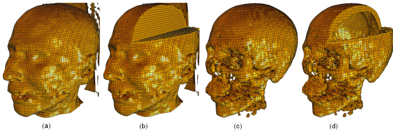
Fig. 20. Quadrilateral and hexahedral meshes are extracted from a CT-scanned volumetric data (UNC head). (a) - the quadrilateral mesh of the skin; (b) - the hexahedral mesh of the volume inside the skin; (c) - the quadrilateral mesh of the skull isosurface; (d) - the hexahedral mesh of the skull.
