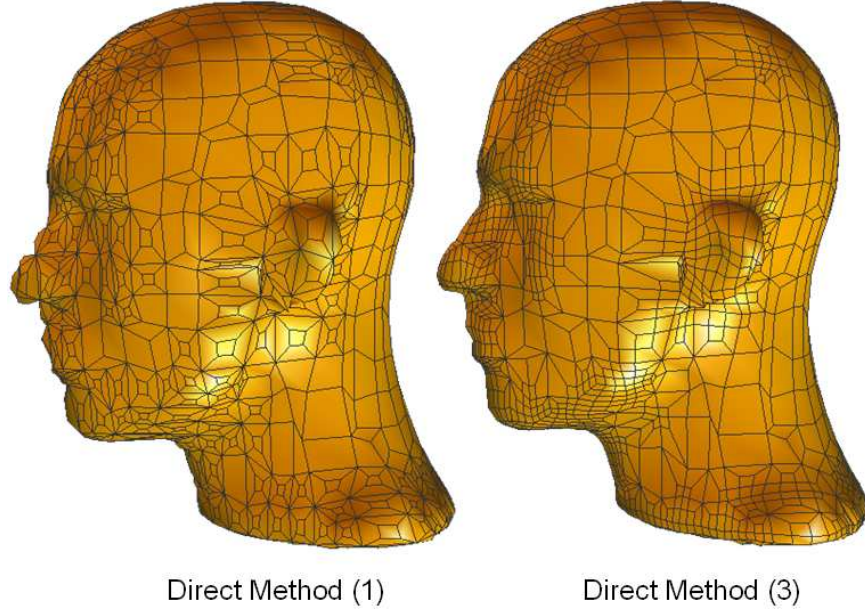
Fig. 7. Adaptive quad meshes generated from two direct methods. A feature sensitive error function [38] [39] is chosen for mesh adaptivity, the isovalue \alpha = 0 , the error tolerance \varepsilon = 0.4 . Method 1 generates a poor nose, and Method 3 generates a better result.
