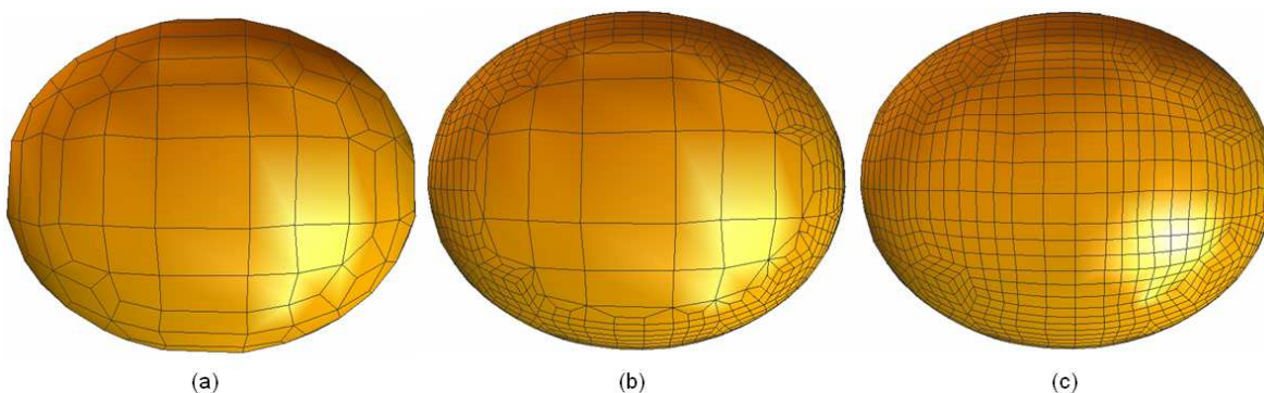
Fig. 21. Quadrilateral meshes of a bubble model. (a) - the uniform mesh at a chosen starting level; (b) - an adaptive mesh controlled by finite element solutions (deformation); (c) - a mesh generated by refining all the elements in (a).
