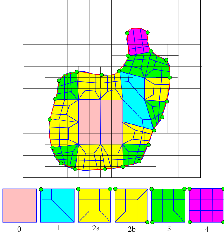
Fig. 8. Top row - an example of adaptive quad mesh generation in 2D. Each green point represents a minimizer point of a cell to be refined, and the red curve represents the real isocontour. Bottom row - the decomposition templates of Method 3 shown in Figure 4.
