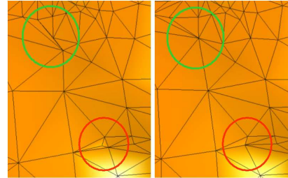
Figure 8: Quality Improvement - Left: no edge contraction, circles mark triangles with bad aspect ratio; Right: poor quality triangles disappear after iterative edge contraction.
