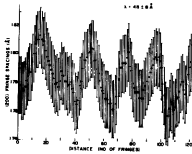
Fig. 3. Periodic variation of lattice fringe spacing in the lattice image of a spinodally decomposed Cu-28.9 Ni-2.8 Cr alloy aged at 700°C for 10 minutes. (38)
