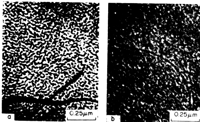
Fig. 20. Spinodal decomposition in the FeAl (B2) ordered phase followed by continuous ordering ( DO_3 ) in the Al-rich regions during aging at 539°C; (a) (222) dark-field showing continuous decomposition of B2, (b) (111) dark-field revealing a high density of fine domains of the DO_3 phase in the Al-rich regions (48). (Note: indexed according to the DO_3 unit cell. See Ref. 48.)
