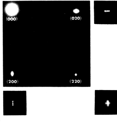
Fig. 11. (a) (002) electron diffraction pattern from a spinodally decomposed Cu-Ti alloy showing the satellite configuration flanking the matrix reflections, (b) schematic showing disposition of satellites in reciprocal space predicted for a triaxially modulated structure, (c) sideband behavior at a (200) reflection in a Cu-2.9 a /o Ti alloy during aging. (7,54)
