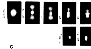
Fig. 12. Sidebands in the X-ray diffraction pattern from a Cu-4 w /o Ti alloy clearly showing symmetrical satellites during the early stages of decomposition and the development of asymmetry in position and intensity after prolonged aging. (60)
