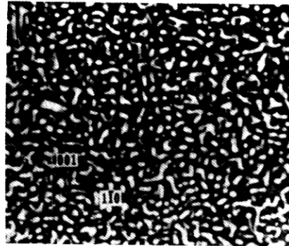
Fig. 17. Isotropic "spinodal microstructure" in an Fe-31 W /o Cr-23 W /o Co alloy aged for one hr at 660°C (92).
