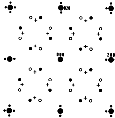
Fig. 10. Schematic of an (002) diffraction pattern of an as-quenched Cu-Ti alloy showing the positions of the \{1\bar{1}0\} diffuse scattering (+), D_1 superlattice reflections (0,2) and satellite spots. (6)
