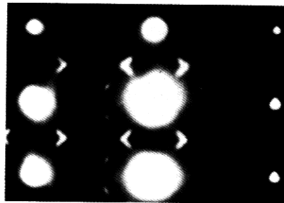
Fig. 15. Ni,Mo alloy aged 10 min. at 650°C. Note the continuous intensity distribution from the {110}'s to the D1 superlattice positions (72). a
