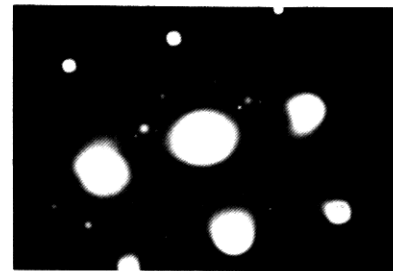
Fig. 13. The [001] pattern of a Ni-16.7 a /o Mo alloy aged at 750°C for 20 min. Sharp LRO reflections are observed at \frac{1}{5} {420}.
