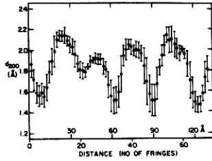
Fig. 5. Variation of the fringe spacing versus distance in the lattice image of the Au-Ni alloy. (39)
