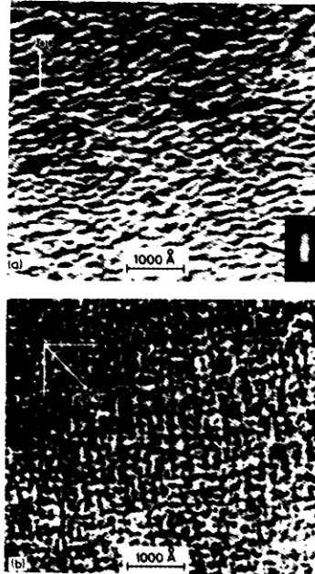
Fig. 2. Triaxially modulated structure developed in a Cu-31.6 Ni-1.7 Cr alloy aged at 650°C for 1 hr revealed by matrix strain contrast striations along the traces of {100} planes (a) \vec{g}=200 (b) \vec{g}=220 ; foil normal near [001].(37)
