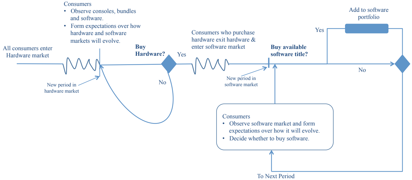
Figure 3: Model Timeline
