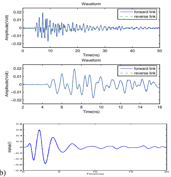
Fig. 3. Channel reciprocity in the engine compartment.
