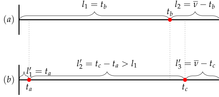
Figure 3: Maximum Step Length and T . (a) Case T = 2 , (b) Case T = 3 .
