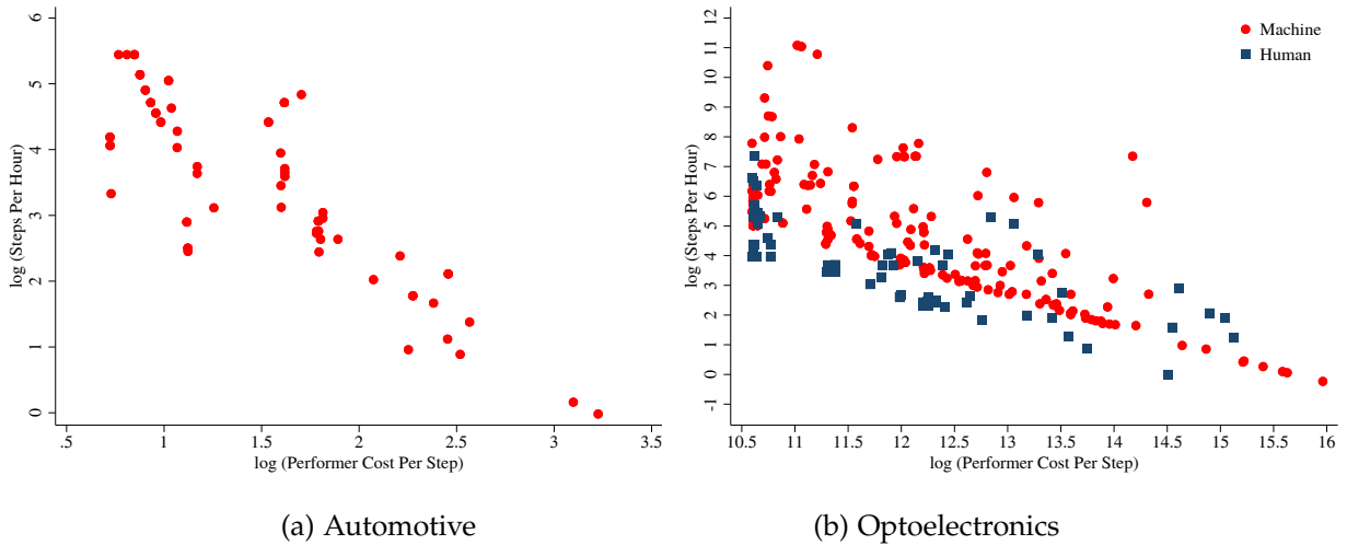
Figure 4: Rates of production and performer costs per step.
